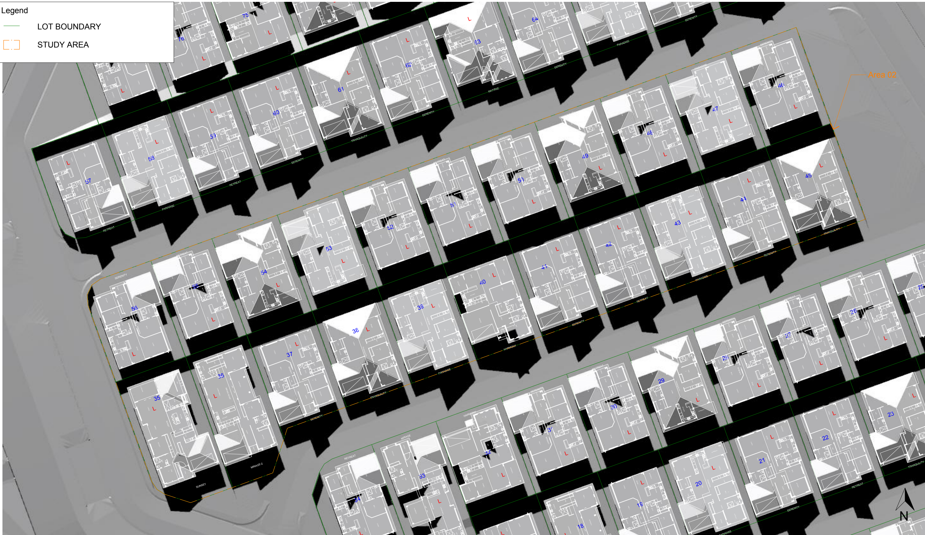
Map Title / Figure: Winter Solstice Shadow Diagrams - Area 02 - 1PM
