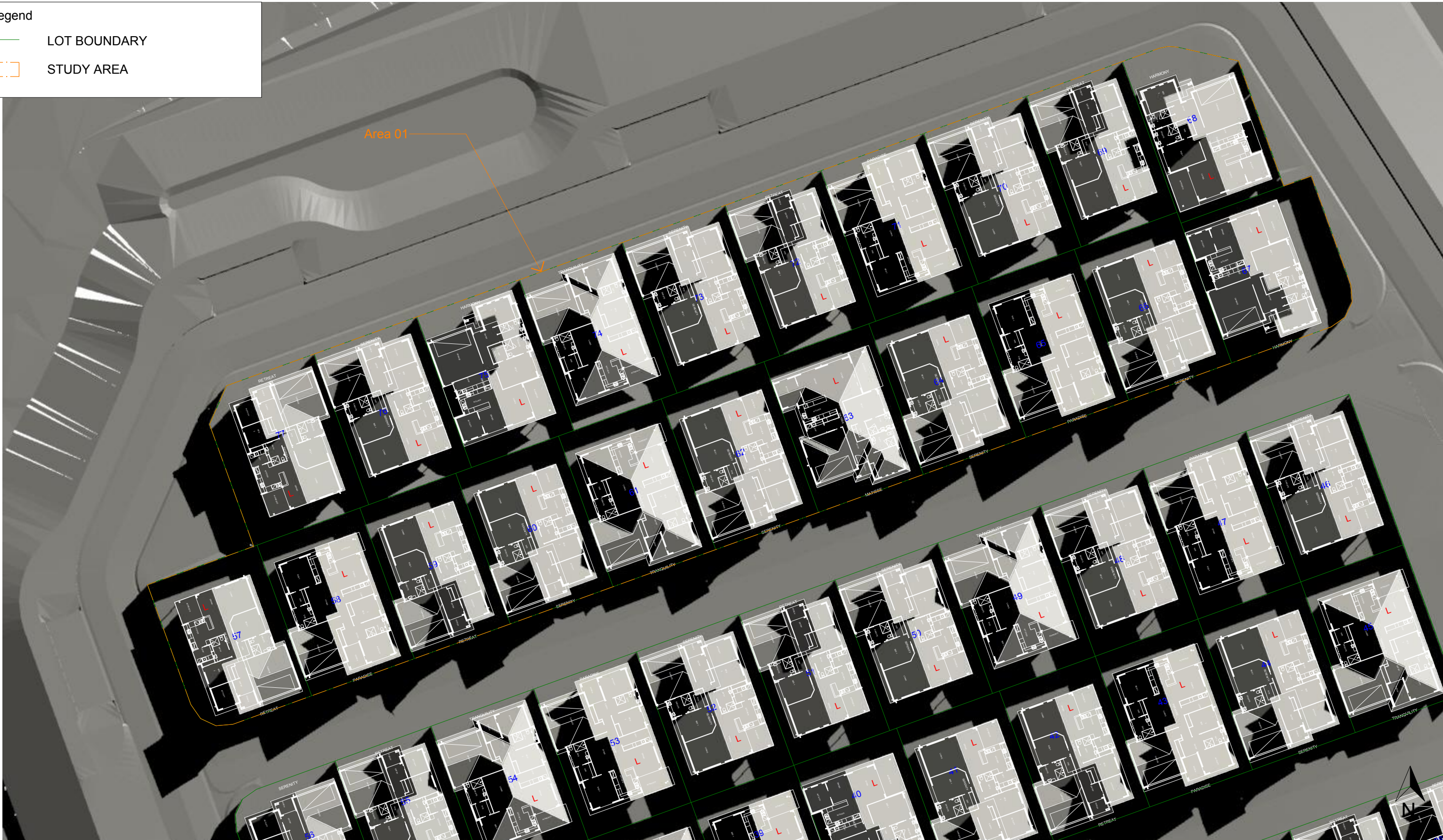
Map Title / Figure: Winter Solstice Shadow Diagrams - Area 01 - 9AM
