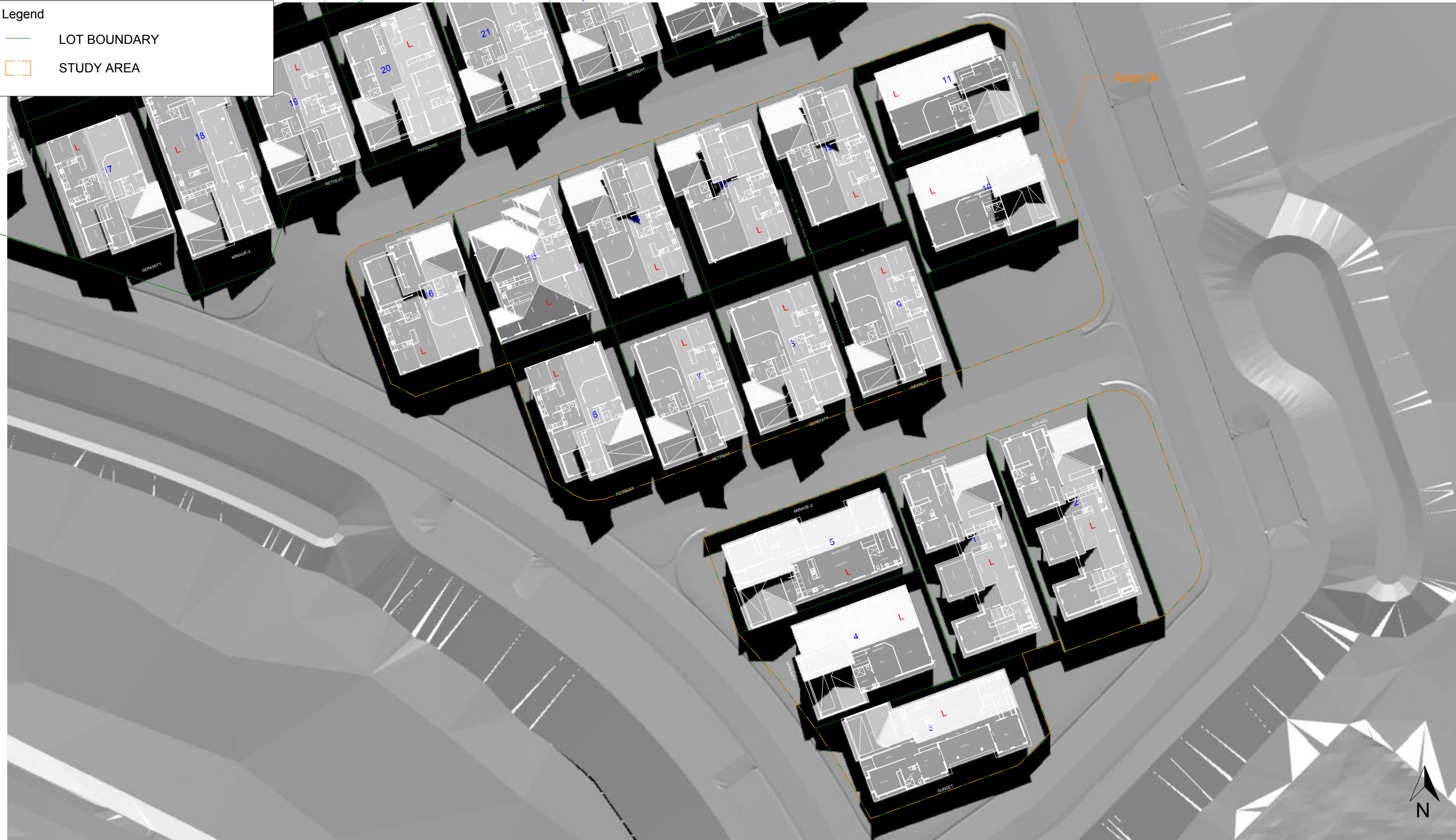
Map Title / Figure: Winter Solstice Shadow Diagrams - Area 04 - 12PM
